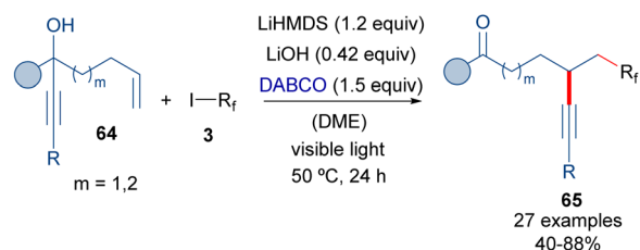
Scheme 10 Transition metal-free radical \alpha -perfluoroalkylation with concomitant \beta -alkynylation of unactivated alkenes. DABCO: 1,4-diazabicyclo[2.2.2]octane.
