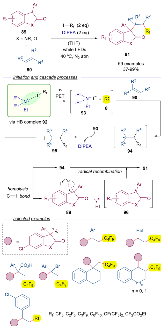
Scheme 14 Photochemical catalyst-free three-component synthesis of polyfluorinated oxindoles 91 .
