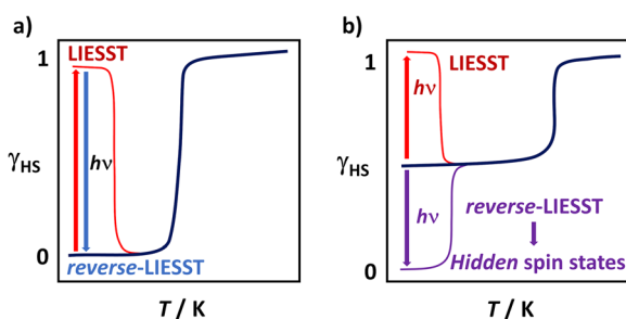
Fig. 1 Visual representation of (a) LIESST and reverse-LIESST and (b) light activation to access hidden (not easily accessible) spin states.
