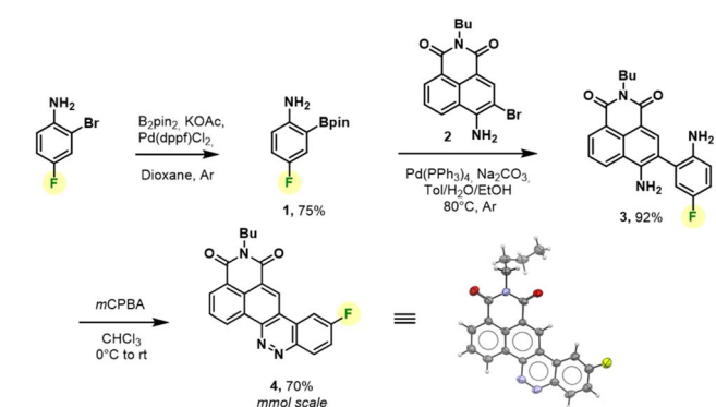
Fig. 2 mmol scalable synthesis and X-ray diffraction structure of bench stable CinNapht-F 4 .
