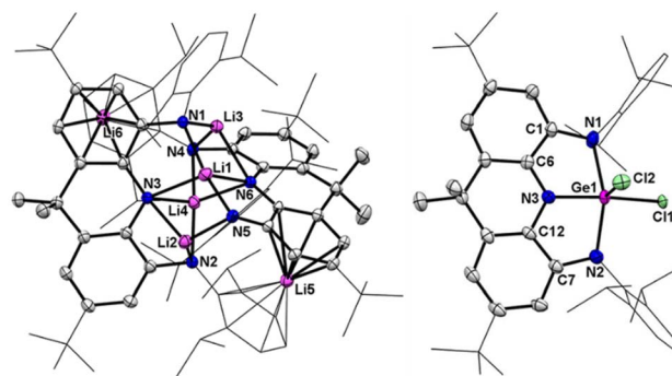
Fig. 2 Left: Solid-state structure of 2 . Right: solid-state structure of 3 . The t Bu and Dipp groups are simplified as wireframes and hydrogen atoms are omitted for clarity. Thermal ellipsoids are set at the 30% probability level. Selected bond lengths (Å) and angles (°) for 2 : Li1–N1 1.890(4), Li1–N3 2.254(4), Li1–N5 1.903(4), Li1–N6 2.236(4), Li2–N2 2.013(5), Li2–N3 2.133(4), Li2–N5 1.992(4), Li3–N1 1.978(4), Li3–N4 2.000(4), Li3–N6 2.157(4), Li4–N2 2.030(4), Li4–N3 2.092(4), Li4–N4 2.038(4), Li4–N6 2.073(4). Selected bond lengths (Å) and angles (°) for 3 : Ge1–Cl1 2.091(2), Ge1–Cl2 2.163(2), Ge1–N1 2.011(2), Ge1–N2 2.039(2), Ge1–N3 1.872(2), C1–N1 1.387(3), C7–N2 1.379(3), C6–N3 1.349(3), C12–N3 1.362(3), C1–C6 1.404(3), C7–C12 1.402(3), N1–Ge1–N2 153.22(10), N1–Ge1–N3 80.34(8), N2–Ge1–N3 79.59(9), Cl1–Ge1–Cl2 104.09(10).
