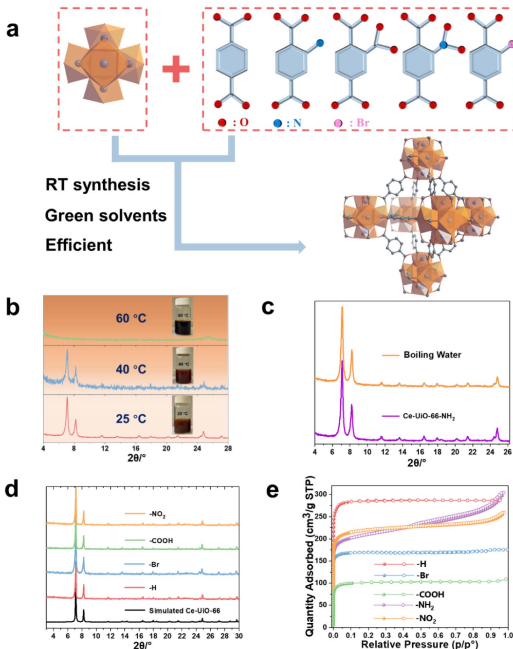
Fig. 1 (a) Crystal structures of Zr 6 oxo-cluster, linkers, and Ce-UiO-66. (b) PXRD ( \lambda_{\text{Cu}} = 1.5406 \text{ \AA} ) patterns of the Ce-UiO-66-NH 2 synthesized at various temperatures (25 °C, 40 °C, 60 °C), insert image: the photograph of the resulting solution. (c) PXRD patterns ( \lambda_{\text{Cu}} = 1.5406 \text{ \AA} ) of the Ce-UiO-66-NH 2 sample before and after boiling water treatment. (d) PXRD patterns ( \lambda_{\text{Cu}} = 1.5406 \text{ \AA} ) of the RT synthesized Ce-UiO-66-X (X = -H, -NO 2 , -COOH, -Br). (e) 77 K N 2 adsorption-desorption isotherms of the RT synthesized Ce-UiO-66-X.
