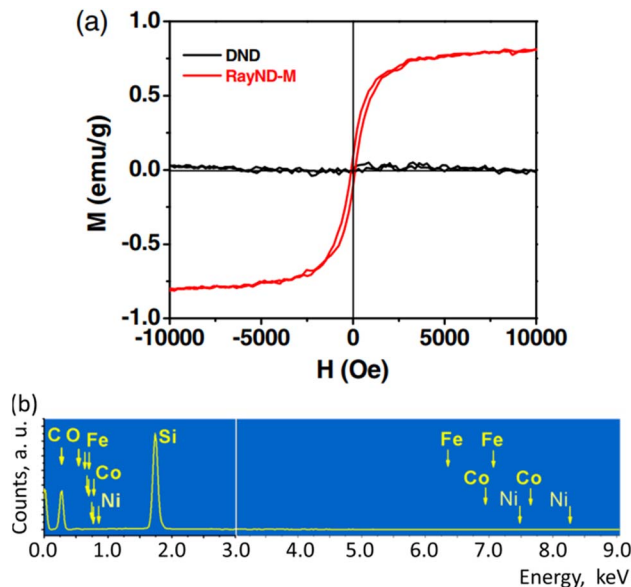
Fig. 10 Magnetic properties of RayND-M ( d = 4.3\text{--}4.5 \text{ nm} ). (a) Magnetization curve of RayND-M [in comparison with ordinary detonation ND (DND), d = 3\text{--}10 \text{ nm} ]. (b) EDS spectrum of RayND-M; Fe, Co, and Ni atoms as impurities were not detected. 139 Reproduced with permission from ref. 139 Copyright 2018 SPIE.
