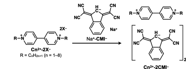
Scheme 1 Preparation of ion pairs comprising 1,1'-dialkyl-4,4'-bipyridinium cations ( \text{C1}^{2+} – \text{C8}^{2+} ) and 1,3-bis(dicyanomethylidene)indan anion ( \text{CMI}^- ).
