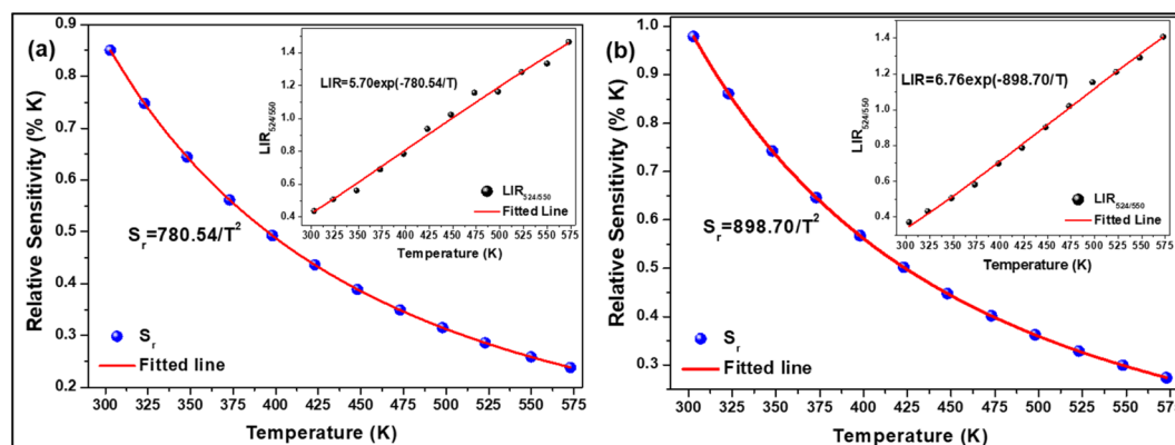
Fig. 4 Relative sensitivity (LIR 524/550 variation) as a function of temperature at (a) 3.76 \text{ W cm}^{-2} , (b) 5.78 \text{ W cm}^{-2} of 7 mol% \text{Er}^{3+} -10 mol% \text{Yb}^{3+}\text{:NaZr}_2(\text{PO}_4)_3 phosphors.
