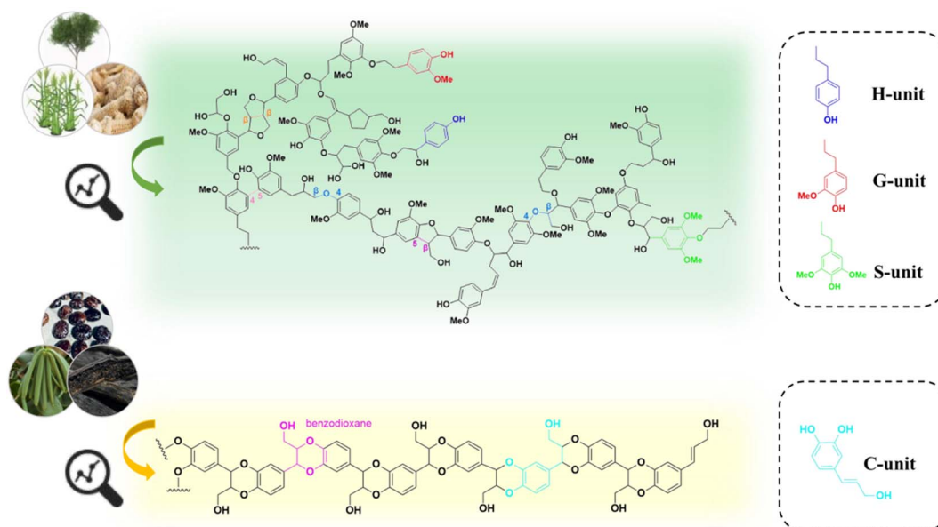
Fig. 1 Proposed structure of H/G/S lignin versus C-lignin revealed by NMR analysis. 15
