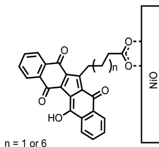
Fig. 9 Schematic representation of KuQ3CO 2 H or KuQ8CO 2 H chemisorption on NiO.
