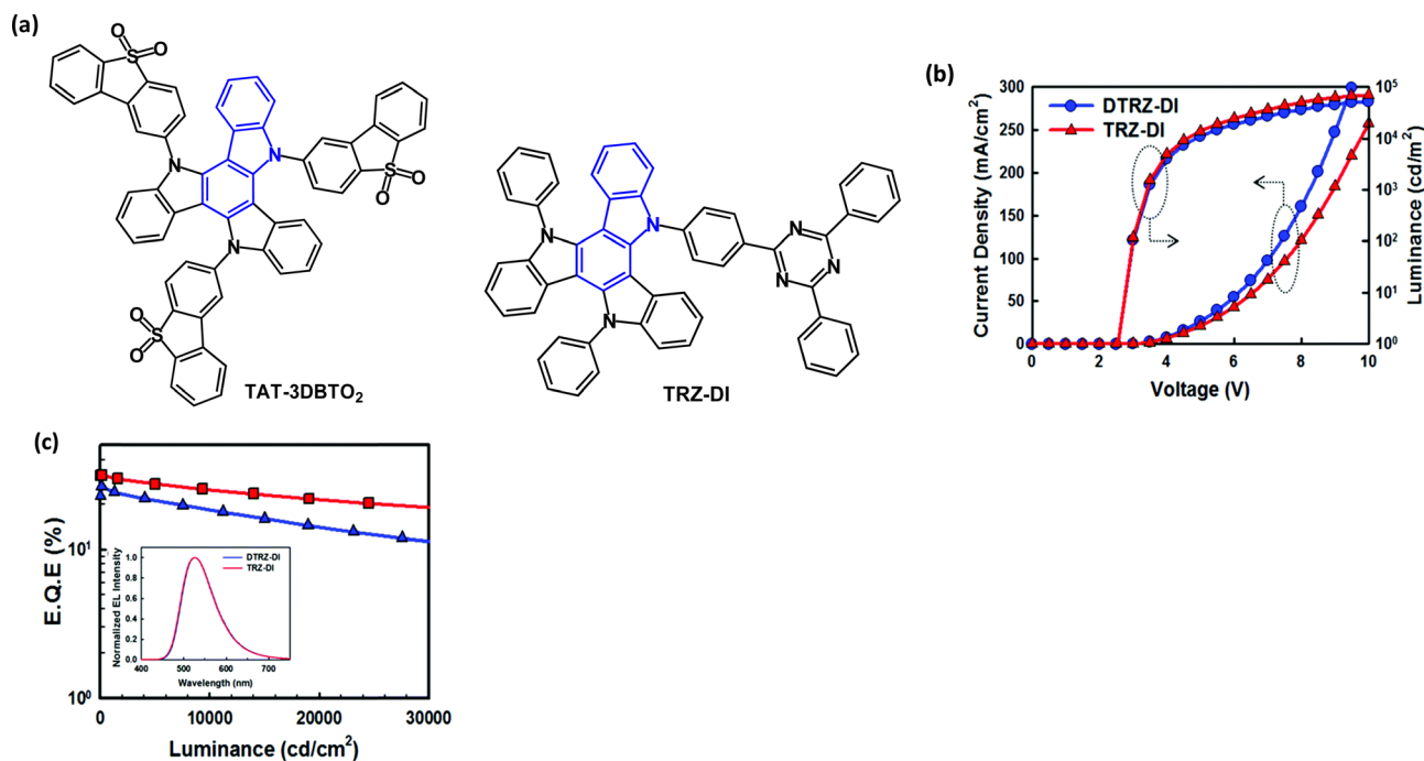
Fig. 24 (a) Molecular structures of TAT-3DBTO 2 and TRZ-DI . (b) Current density–voltage–luminance ( J – V – L ) data. (c) \text{EQE} – L data; inset EL spectra for TRZ-DI and DTRZ-DI devices. 140 Copyright 2018 The Royal Society of Chemistry.
