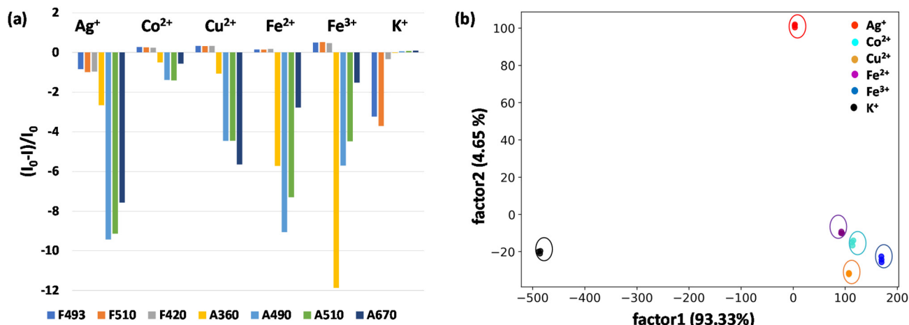
Fig. 5 (a) The absorption and fluorescence response patterns of six metals with D1 and (b) a LDA plot obtained from the absorbance and fluorescence responses of D1 with \text{Ag}^+ , \text{Cu}^{2+} , \text{Co}^{2+} , \text{Fe}^{2+} , \text{Fe}^{3+} and \text{K}^+ .
