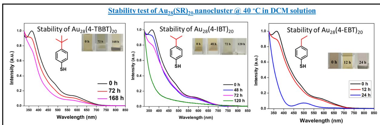
Fig. 4 UV-visible absorption spectra showing the stability test of Au 28 (SR) 20
