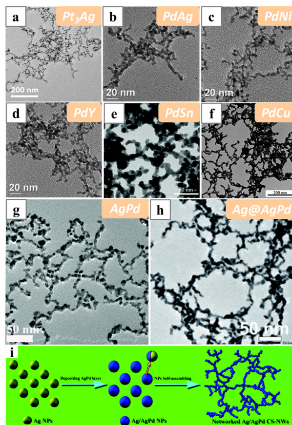
Fig. 15 TEM images of (a) \text{Pt}_3\text{Ag} , (b) PdAg, (c) PdNi, (d) PdY, (e) PdSn, (f) PdCu, (g) AgPd and (h) Ag@AgPd nanowires synthesized with PVP as the structure-directing reagent in aqueous solutions. (i) Schematics illustrating the oriented attachment of Ag@AgPd nanoparticles into networked Ag@AgPd nanowires. Reprinted with permission from ref. 127–129, 131, 133 and 134. Copyright 2020 from Springer Nature, 2018 and 2021 from the Royal Society of Chemistry, 2017 from Elsevier.
