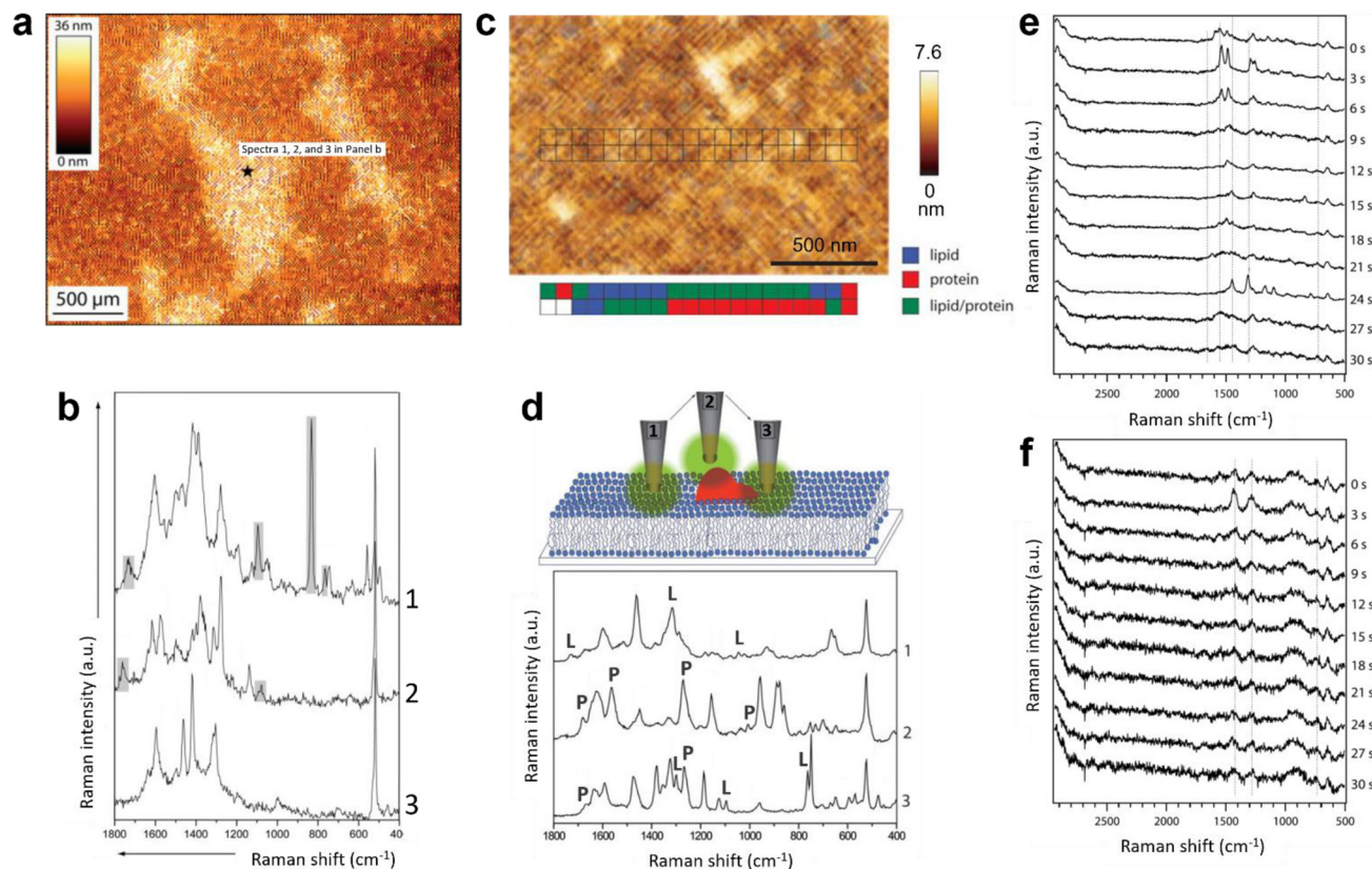
Fig. 3 (a) AFM topography image of a POPC/DOPS bilayer on mica. TERS spectra were recorded at the marked spot (black star). (b) TERS spectra measured consecutively at the spot marked in panel (a). Panels (a) and (b) are adapted from ref. 49 with permission from John Wiley & Sons, copyright 2009. (c) AFM topography image of a streptavidin-labelled phospholipid film. The positions where TERS spectra were recorded are marked. A false-colour map of the lipid and protein regions is shown below the topography image. (d) Schematic diagram illustrating different tip-sample interactions during the TERS measurement of the streptavidin-labelled phospholipid film and a plot of the corresponding TERS spectra. Marker bands for lipids and proteins are labelled with L and P, respectively. Panels (c) and (d) are adapted from ref. 50 with permission from John Wiley & Sons, copyright 2010. Time-series TERS spectra of supported (e) DOPC and (f) DPPC bilayers. Panels (e) and (f) are adapted from ref. 51.
