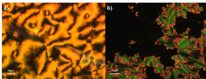
Fig. 4 Textures observed for the mO.O5O.Om series: (a) schlieren texture of the nematic phase ( T = 163^{\circ}\text{C} ) for 5O.O5O.O5 and (b) focal conic fan texture with homeotropic regions of the smectic A phase ( T = 165^{\circ}\text{C} ) for 9O.O5O.O9.
