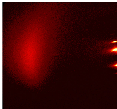
Fig. 5 2D X-ray diffraction pattern for 9O.O5O.O9 in the smectic A phase ( T = 150^{\circ}\text{C} ).
