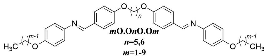
Fig. 3 The molecular structure of the m\text{O}.O_n\text{O}.O_m family of dimers.
