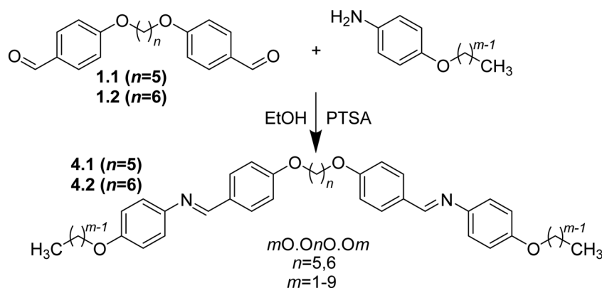
Scheme 2 Synthesis of the m\text{O}.O_n\text{O}.O_m series.
