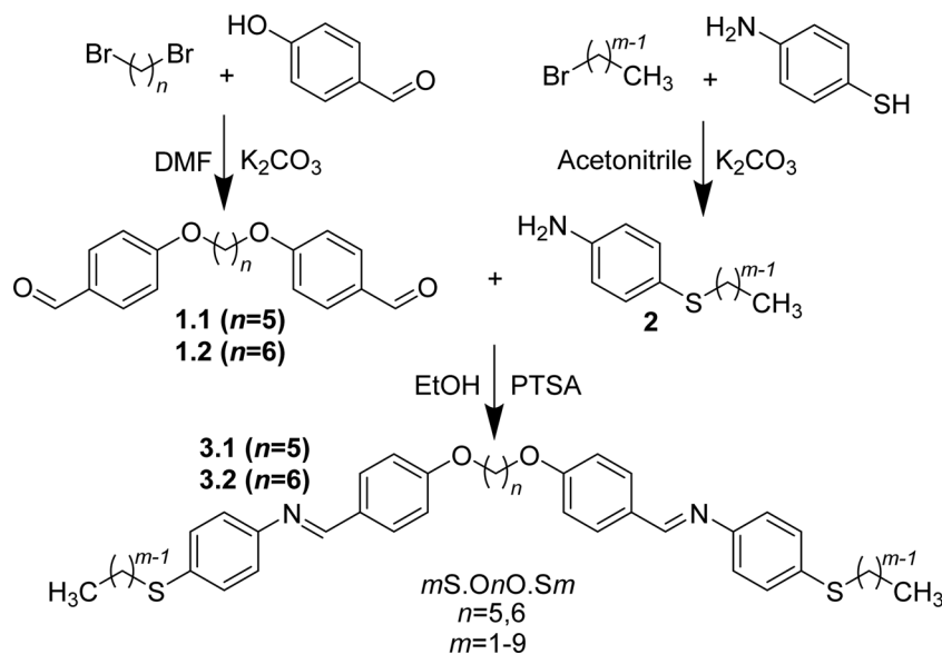
Scheme 1 Synthesis of the m\text{S}.O_n\text{O}.S_m series.
