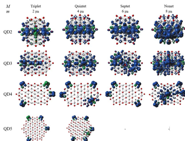
Fig. 8 Spin density for different sizes and spin multiplicities of \text{Ti}_2\text{CO}_2\text{-O} QDs. The isosurface values are 0.002 \text{ e}/\text{bohr}^3 (blue color represents positive and green color represents negative spin density). Titanium, carbon and oxygen atoms are shown in light grey, dark grey and red, respectively. Septet and nonet for QD5 are not calculated.
