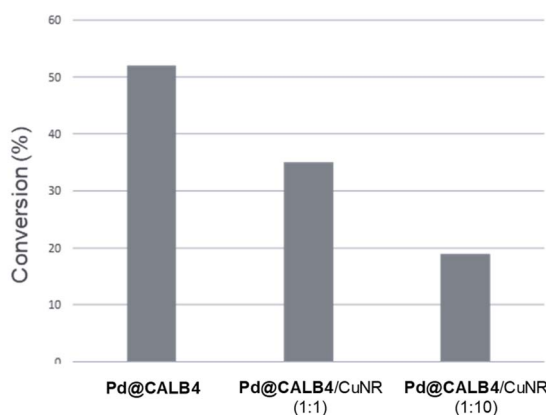
Fig. 4 Application of Pd@CALB4 and Cu biohybrid for the C–H activation of 1 using iodobenzene ( 4 ). Reaction Conditions: 1 (0.046 mmol), 4 (0.1029 mmol), solvent (1 mL), 24 h at r.t. (ca. 21 °C). Conversion of product 5 was quantified by HPLC.
