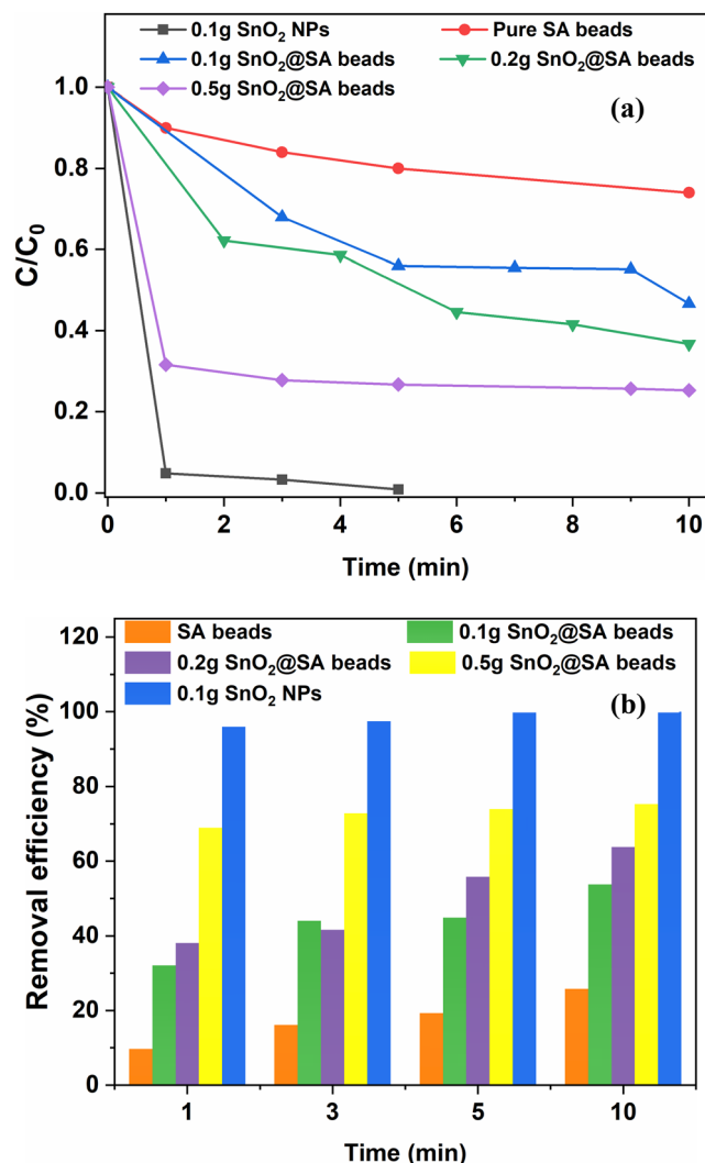
Fig. 10 (a) Various compositions of \text{SnO}_2 @SA beads for CR dye adsorption, and (b) their comparative analysis through a bar diagram.
