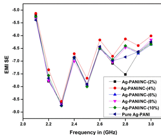
Fig. 8 Frequency vs. EMI SE of Ag-PANI, and Ag-PANI/NC composites of 2, 4, 6, 8 & 10%.
