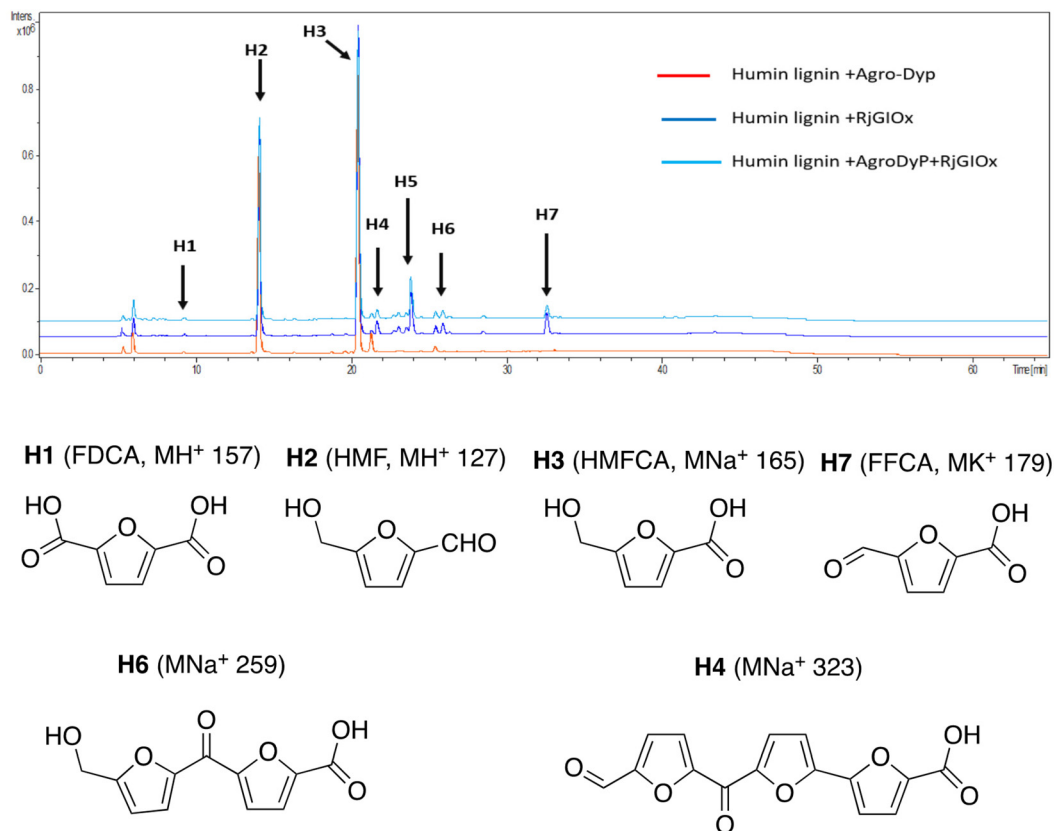
Fig. 8 Total ion chromatogram of products from bioconversion of Avantium humins by AgroDyP and RjGIOx. Structures for H1–H3 and H7 confirmed by co-elution with authentic standards, structures for H4 and H6 based on predicted humin structure. 30
