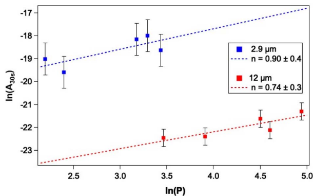
Fig. 9 Plot of \ln(A_{30.5}) as a function of \ln(P) to determine the laser power dependence of irradiation of mixed CO–water ices, comprising 13.3% CO with respect to 780 L m water ice dosed on Au-coated Cu at 18 K, at 2.9 \mu\text{m} and 12 \mu\text{m} for 5 minutes. Within the errors, excitation at both wavelengths is consistent with a single-photon process.
