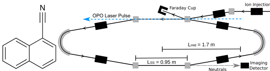
Fig. 1 (Left) Structure of 1-cyanonaphthalene ( \text{C}_{10}\text{H}_7\text{CN} , 1-CNN). (Right) Schematic of DESIREE storage ring.
