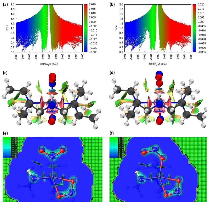
Fig. 6 Non-covalent interaction (NCI) analysis for the GS and ES isomers of 2, using the reduced density gradient (RDG, s ). Theoretical analysis: (a) plot of s vs \text{sign}(\lambda_2\rho) for GS nitro- (\eta^1\text{-NO}_2) and (b) plot of s vs \text{sign}(\lambda_2\rho) for ES nitro- (\eta^1\text{-ONO}) , providing a fingerprint of the NCIs in each isomer [generated in Multiwfn 25 and visualised in GnuPlot 33 ]. (c) 3D plot of s isosurfaces ( s = 0.5 a.u.) for GS nitro- (\eta^1\text{-NO}_2) and (d) 3D plot of s isosurfaces ( s = 0.5 a.u.) for ES nitro- (\eta^1\text{-ONO}) , highlighting the key NCIs in each isomer: colour-coding links to (a)/(b) plots with red = regions of \text{sign}(\lambda_2\rho) > 0 i.e. steric interactions, green = regions of \text{sign}(\lambda_2\rho) \approx 0 and blue = regions of \text{sign}(\lambda_2\rho) < 0 i.e. bonding interactions e.g. hydrogen bonds [generated in Multiwfn and visualised in VMD 26 ]. HAR analysis: (e) 2D s (RDG) map for the GS structure of 2 in the Ni(1), N(1), O(1), O(2) plane and (f) 2D s (RDG) map for the ES structure of 2 in the Ni(1), O(1A), N(1A), O(2A) plane, showing key NCIs in the asymmetric unit [generated by HAR in NoSpherA2 9 ].
