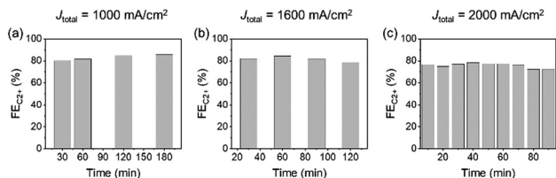
Fig. 5 \text{FE}_{\text{C}_{2+}} stability tests with respect to the current density over CuONPs-1.0/GDE in 1 M KCl under (a) J_{\text{total}} = 1000 \text{ mA cm}^{-2} , (b) 1600 \text{ mA cm}^{-2} and (c) 2000 \text{ mA cm}^{-2} .
