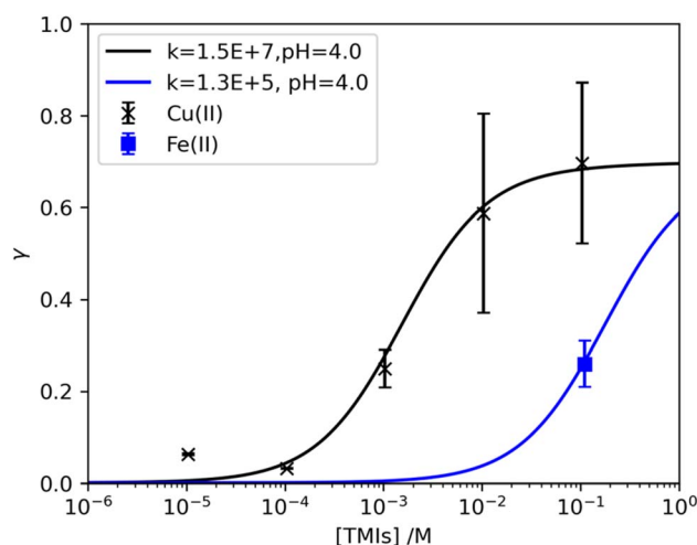
Fig. 5 HO 2 uptake coefficient as a function of the estimated [TMIs] in the aerosol phase. The solid lines represent the resistance model estimated with r_p = 85 nm, [HO 2 ] = 1 × 10 10 molecules cm −3 , and \alpha = 0.7.
