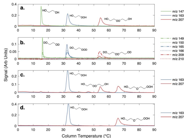
Fig. 2 (a) GC traces of three products of the ethene oxidation experiments: ethylene glycol ( m/z 147), accretion product ( m/z 207), and ROOH ( m/z 163). (b) GC traces with D 2 O added to flow tube. Dashed lines are signals at m/z + 2 for each product shown in a, and dotted lines are the signals at m/z + 3 for each product. Solid lines are signals at each original product m/z . (c) GC traces of m/z 163 and m/z 207 from the synthesized standard prior to prep TLC purification. (d) GC traces of m/z 163 and m/z 207 from the standard after purification by preparatory TLC.
