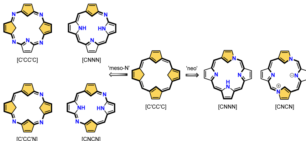
Scheme 132 Convoluted inner core/meso- or \alpha -C perimeter four nitrogen atom "nitriding" of quaterin to generate neo-confused and di-neo-confused porphyrins or meso-aza-carbaporphyrins (an inner core described as: [set donor atoms], hybridisations: C' tetrahedral, C trigonal, and N trigonal).
