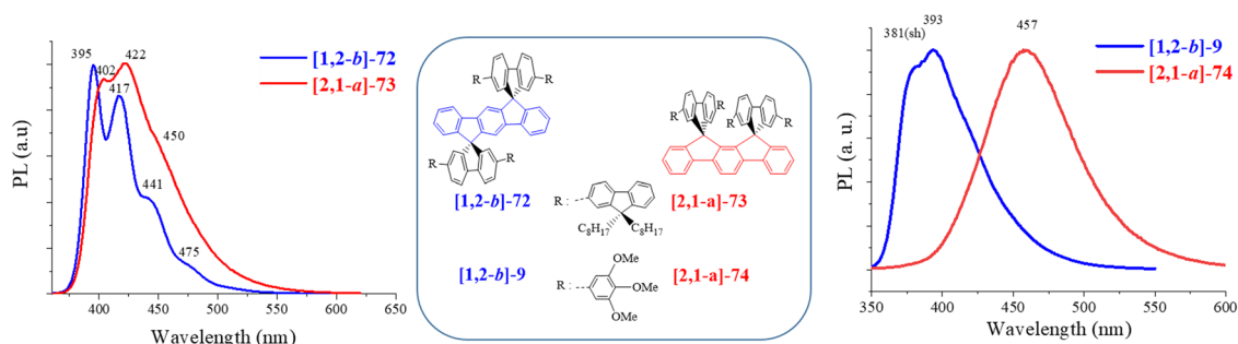
Fig. 10 [2,1- a ]DHIF-based organic semiconductors used as the EML in fluorescent OLEDs ([2,1- a ]-73 and [2,1- a ]-74) and their respective [1,2- b ]-isomers ([1,2- b ]-72 and [1,2- b ]-9), fluorescent spectra of the four compounds.
