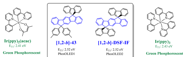
Fig. 6 [1,2- b ]DHIF -based organic semiconductors used as the host for phosphorescent dopants in PhOLEDs ( [1,2- b ]-43 and [1,2- b ]-DSF-IF ) and green phosphorescent \text{Ir}(\text{ppy})_2(\text{acac}) and \text{Ir}(\text{ppy})_3 .
