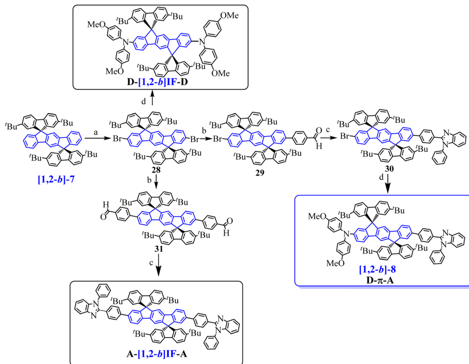
Scheme 9 Synthesis of [1,2- b ]-8, and of its parent A-[1,2- b ]IF-A and D-[1,2- b ]IF-D derivatives. (a) Br 2 , Na 2 CO 3 , I 2 (catalytic amount), CH 2 Cl 2 /water, RT, (90%); (b) Pd 2 (dba) 3 /P( t Bu) 3 , Na 2 CO 3 , 4-formylphenylboronic acid (1.4 eq. vs. 28 for 29 or 2 eq. vs. 28 for 31 ), toluene/water, 100 °C; (c) methoxyethanol, N -phenyl- o -phenylenediamine, 120 °C; (d) Pd(OAc) 2 , P( t Bu) 3 , t BuOK, 4,4'-dimethoxydiphenylamine, toluene, 100 °C.
