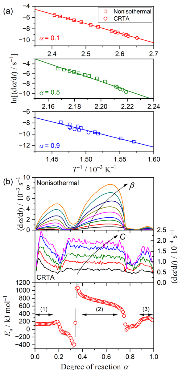
Fig. 4 Results of isoconversional kinetic analysis for the overall thermal dehydration of DCPD (63–75 μm) in a stream of dry N 2 : (a) Friedman plot at different \alpha values, and (b) changes in (d\alpha/dt) as the reaction advances under linear nonisothermal and CRTA conditions, and E_a values at different \alpha .
