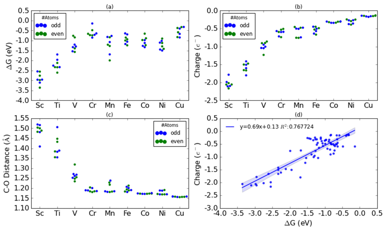
Fig. 4 (a) \text{CO}^* adsorption free energies ( \Delta G , eV), (b) residual charge ( e^- ) on \text{CO}^* , (c) C-O bond distances ( \text{\AA} ) in \text{CO}^* , and (d) correlation between \text{CO}^* adsorption free energies and residual charges on \text{CO}^* for various Sc-Cu nanoclusters. Residual charge indicates the total Bader charge density resides on CO moiety on binding on cluster moiety.
