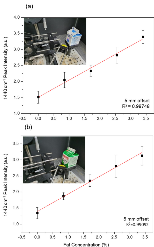
Fig. 5 Quantitation curves of fat concentration in (a) blue and (b) green milk cartons obtained from 5 mm SORS spectra of unopened cartons; the 785 nm laser power was maintained at 300 mW and the exposure time was 10 s with 10-time averaging.
