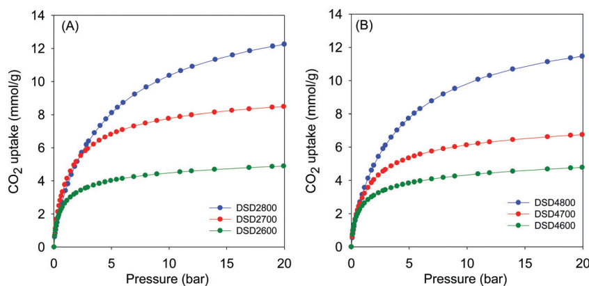
Fig. 4 CO 2 uptake isotherms of carbons directly activated from sawdust (SD) at 600, 700 or 800 °C, and PO/SD ratio of 2 (A) or 4 (B).
