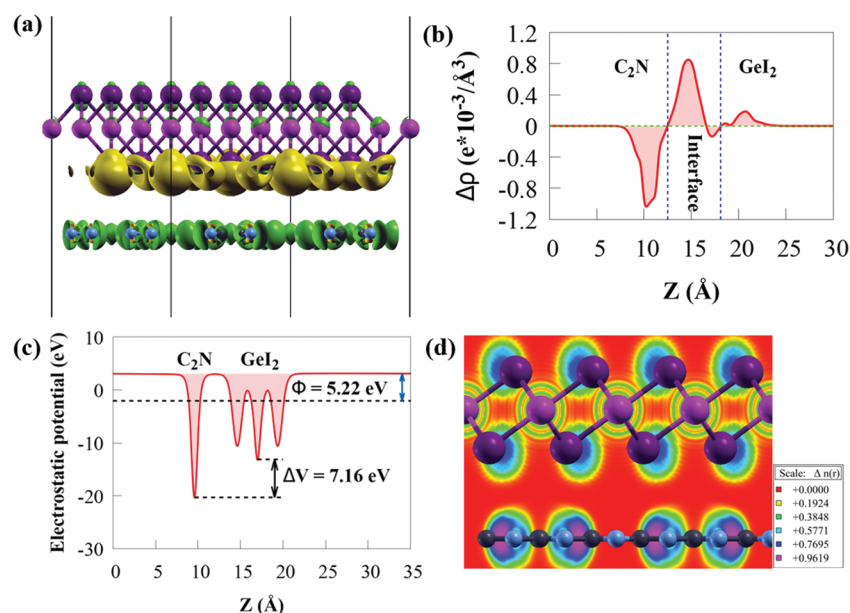
Fig. 4 (a) Three-dimensional charge density difference of the GeI 2 /C 2 N vdW heterostructure with an isovalue of 0.0008 \text{ e bohr}^{-3} . Green and yellow isosurfaces denote charge depletion and accumulation, respectively. (b) The averaged difference in the electron density for the GeI 2 /C 2 N vdW heterostructure along the z-axis. The inner surfaces of the two materials are marked with a blue dashed line. (c) The potential drop ( \Delta V ) for the GeI 2 /C 2 N vdW heterostructure. (d) Electron localisation functions across the GeI 2 /C 2 N vdW heterostructure interface. Grey, blue, magenta and purple balls denote C, N, Ge and I atoms, respectively.
