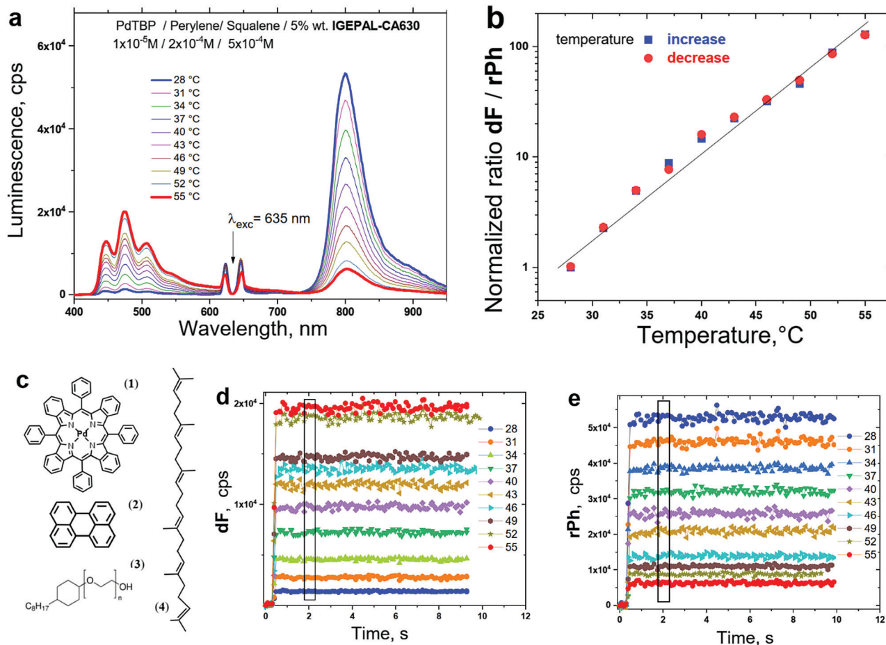
Fig. 15 (a) Dependence of the luminescence spectra of the micellar TTA-UC system. Material composition is as follows, PdTBP/perylenes/squalene/IGEPAL-CA630 in an aquatic environment on the sample temperature. The concentrations of the active materials are as follows, 1 \times 10^{-5} M/ 2 \times 10^{-4} M/ 5 \times 10^{-4} M/5 wt% in water; (b) temperature calibration curve: ratiometric response, representing the normalized ratio of the delayed upconverted fluorescence and residual sensitizer phosphorescence as function of the sample temperature; (c) structure of the active materials, as follows: (1) meso -tetraphenyl-tetrabenzoporphine Palladium (PdTBP); (2) dibenz[ de,k ]anthracene (perylenes); (3) octylphenyl-polyethylene glycol (IGEPAL-CA630); (4) 2,6,10,15,19,23-Hexamethyl-2,6,10,14,18,22-tetracosahexaene (squalene); (d) temporal dependence of the delayed fluorescence for different sample temperatures; (e) temporal dependence of the residual phosphorescence for different sample temperatures. Conditions: the excitation intensity is constant, 100 \text{ mW} \times \text{cm}^{-2} for all measurements; cw – diode laser \lambda = 635 \text{ nm} ; excitation spot diameter – 1000 \mu\text{m} ; sample thickness – 400 \mu\text{m} ; an oxygen-free environment (the samples are prepared and sealed in nitrogen-filled glove-box, 2 ppm \text{O}_2 residual concentration).
