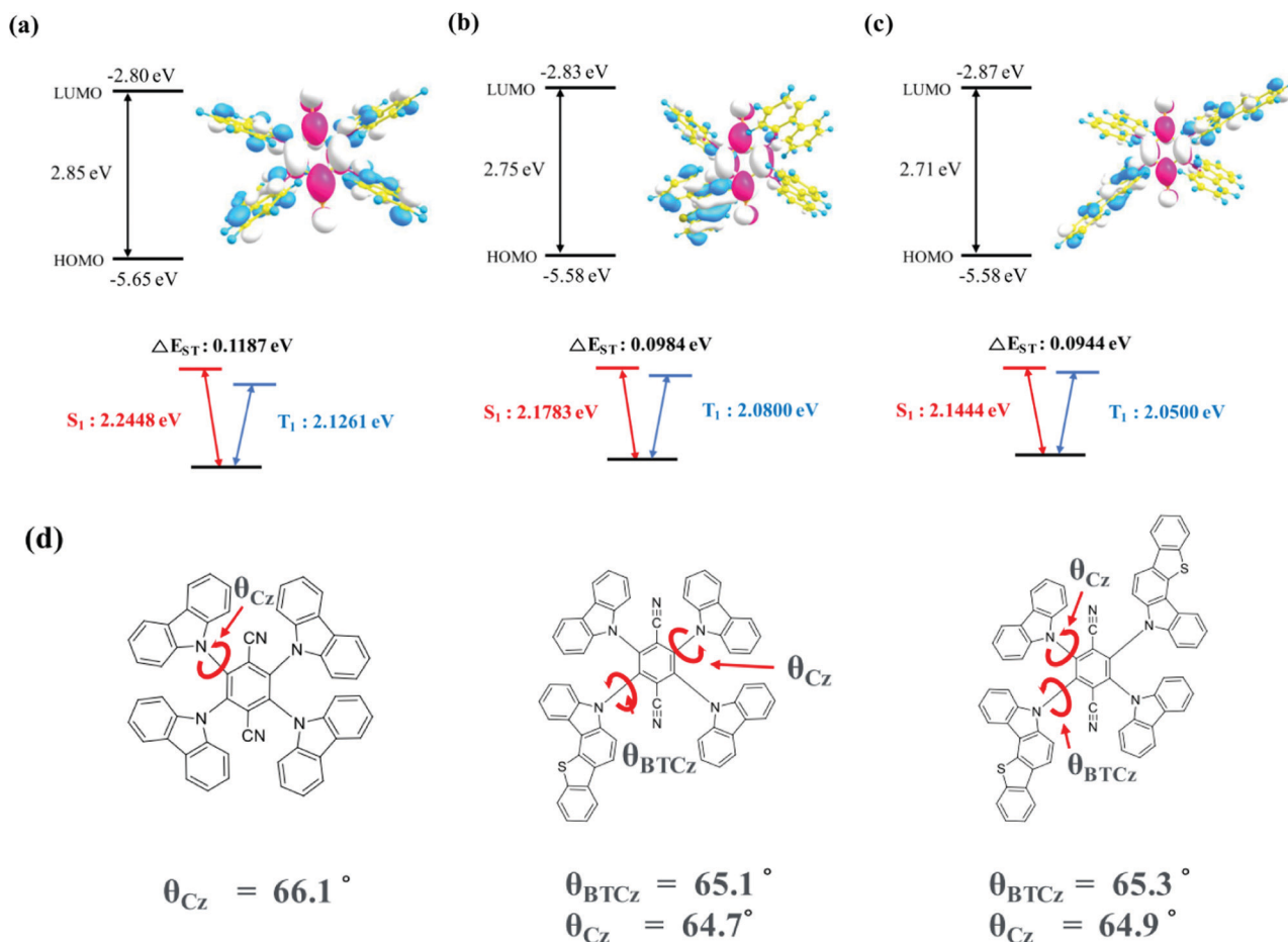
Fig. 1 Optimized ground state HOMO (blue) and LUMO (red) distribution and calculated energy details of (a) 4CzTPN, (b) BTCz 3 CzTPN and (c) 2BTCz 2 CzTPN. (d) Dihedral angles of the Cz and BTCz moieties in 4CzTPN, BTCz 3 CzTPN and 2BTCz 2 CzTPN.
