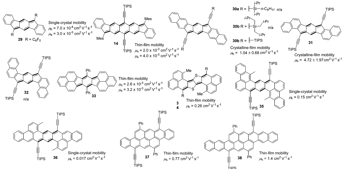
Fig. 7 Open-shell diradicaloids for organic electronics.
