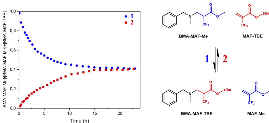
Fig. 1 Kinetic monitoring of BMA-MAF-TBE and BMA-MAF-Me exchange reactions at 1 M by ^{19}\text{F} -NMR in \text{DMF-d}_7 at 60 °C.
