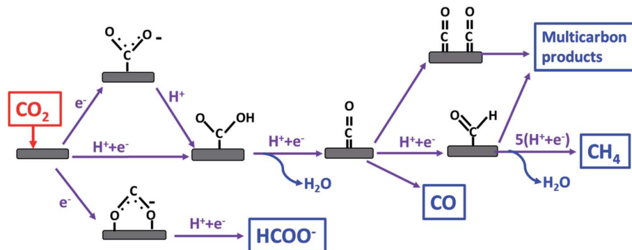
Fig. 1 Scheme of the \text{CO}_2 reduction pathway toward different reaction products.
