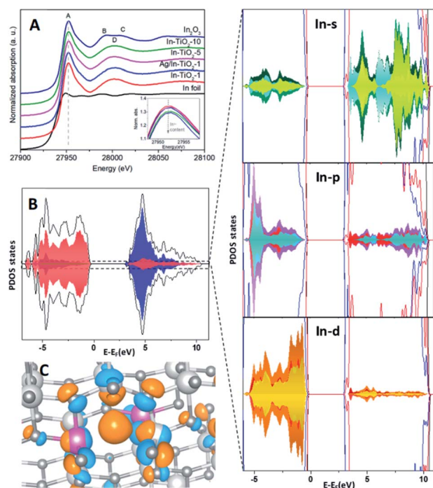
Fig. 4 (A) In K-edge XANES spectra of In-doped \text{TiO}_2 samples and references. The inset shows the decrease of the whiteline (feature A) intensity with In content. (B) Projected density of states (PDOS) for In-doped anatase with oxygen vacancies including In orbitals for each In atom. (C) Spin density plot showing the localization of electrons after formation of an oxygen vacancy in \text{In}_x\text{Ti}_{1-x}\text{O}_{2-y} . Positive values (orange), negative (blue). Colour palette for DOS graphics: In Total DOS profiles (b) O 2p (red), Ti 3d (dark blue), In (yellow); for In PDOS orbitals: In-s total (green), In near to \text{O}_v (yellow), In far to \text{O}_v (cyan); In-p total (violet), In near to \text{O}_v (red), In far to \text{O}_v (cyan); In-d total (orange), In near to \text{O}_v (yellow), In far to \text{O}_v (red).
