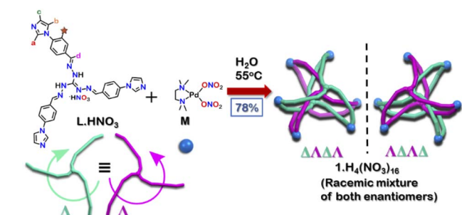
Scheme 1 Synthesis of interlocked Pd 6 cage 1 using a triimidazole donor L \cdot HNO_3 .
