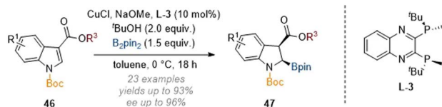
Scheme 14 Enantioselective borylation of C-3 substituted indoles through copper catalysis. 19
