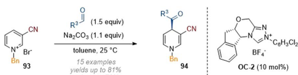
Scheme 27 Enantioselective dearomative C-4 acylation of 3-cyano pyridiniums using NHC catalysis. 33
