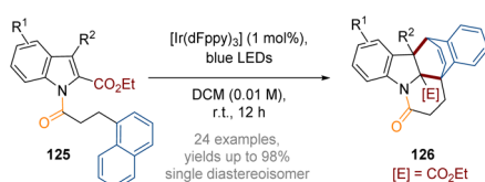
Scheme 36 Visible-light-induced intramolecular double dearomative cycloaddition of arenes. 42
