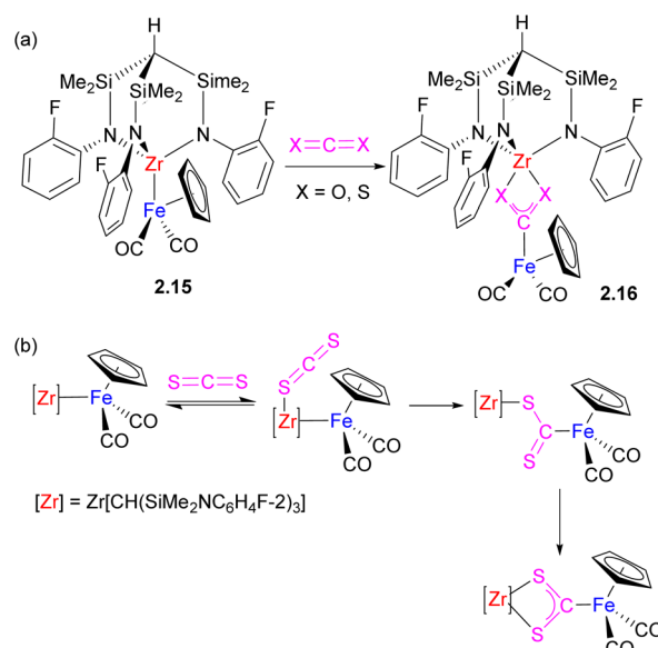
Scheme 8 (a) Insertion of \text{CO}_2 and \text{CS}_2 into unsupported Fe–Zr bond. (b) Proposed mechanism of \text{CS}_2 insertion.
