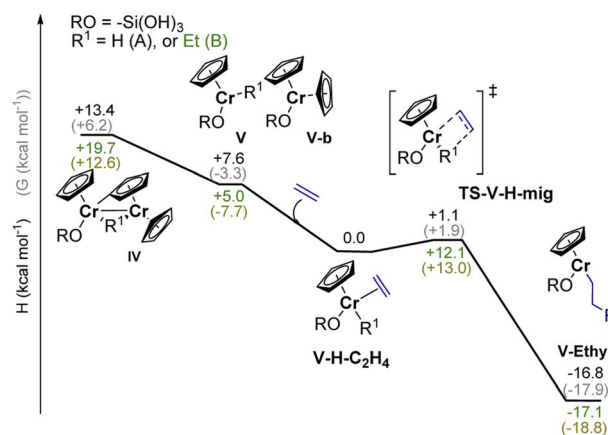
Fig. 5 Calculated reaction enthalpies ( H \text{kcal mol}^{-1} ) and free energies ( G \text{kcal mol}^{-1} ) for potential ethylene activation pathways involving monomeric \text{Cr(III)} hydrides such as V (in black), or monomeric \text{Cr(III)} alkyl species such as V-ethyl (in green). Ethylene activation and chain propagation are both associated with reasonable energy costs.
