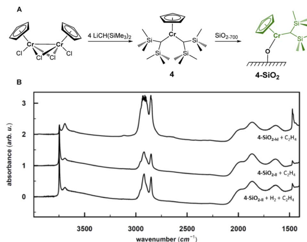
Fig. 6 (A) Synthesis and surface chemistry of 4-SiO 2 . (B) IR spectra of 4-SiO 2 with high Cr loading (0.8 wt%) after exposure to 25 mbar of \text{C}_2\text{H}_4 (top), and 4-SiO 2 with low Cr loading (0.2 wt%) after exposure to \text{C}_2\text{H}_4 (middle) and \text{H}_2 (50 mbar) prior to \text{C}_2\text{H}_4 (bottom). The higher intensity of C–H bands after exposure of the low Cr-loading material to \text{H}_2 evidences for slightly higher EP activity.
