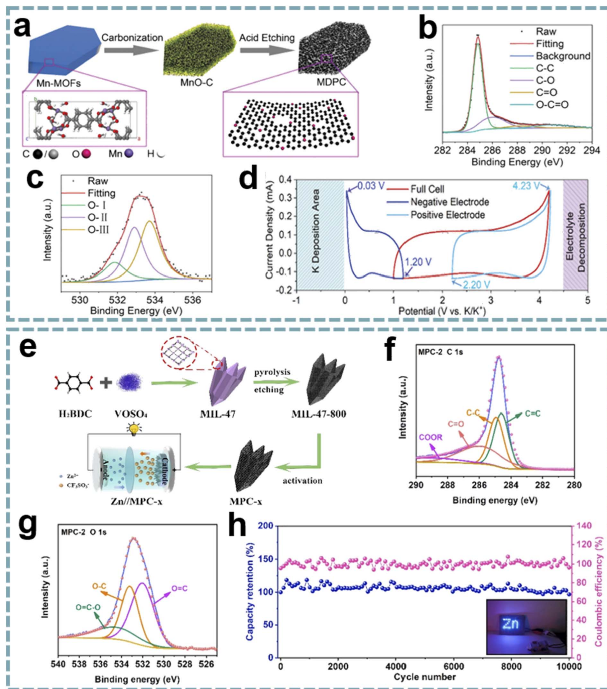
Fig. 9 MOF-derived oxygen-functional carbons for MIHCs. (a) Schematic diagram of the synthesis of a MDPC. (b) C 1s and (c) O 1s XPS spectra of the MDPC. (d) CV profiles based on a three-electrode device at 2 \text{ mV s}^{-1} . Reproduced with permission from ref. 185. Copyright 2020, Wiley-VCH. (e) Synthesis schematic of MPC and construction of Zn//MPC-x ZIHC. High-resolution XPS spectra of (f) C 1s and (g) O 1s of MPC-2. (h) Cycling performance and coulombic efficiency at 10 \text{ A g}^{-1} of the Zn//MPC-2 ZIHC device. Reproduced with permission from ref. 186. Copyright 2021, Elsevier.
