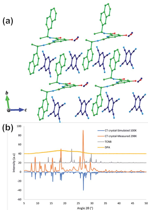
Fig. 7 (a) Extended structure of the CT complex featuring numerous \pi \cdots \pi stacking interactions between the naphthalene ring and TCNB guest molecules. Hydrogen atoms are omitted for clarity. DPA's C atoms are coloured in green and TCNB's C atoms are coloured in deep blue; O is in red, and N is in sky blue for both DPA and TCNB. (b) X-ray powder diffraction pattern for the DPA–TCNB CT complex collected at 298 K compared to those of DPA and TCNB and the calculated pattern from the single crystal dataset of the DPA–TCNB co-crystal at 100 K.
