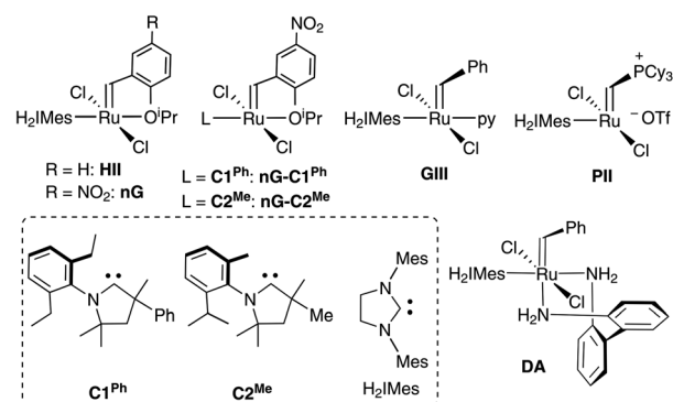
Chart 1 Catalysts and carbene ligands discussed. The CAAC labelling system adopted 42 (C # R ) numbers these ligands by common NAR moiety. The superscript R specifies the variable substituent on the quaternary site α to the carbene carbon.
