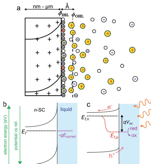
Fig. 3 (a) Scheme of the space charge layer in an n-SC (left) and the Helmholtz layer at the SC/liquid interface (right), adapted with permission from ref. 92 \phi_{IHL} and \phi_{OHL} are the inner and the outer Helmholtz planes. (b) Scheme showing a depleted n-SC in equilibrium with an electrolyte containing the ox/red redox couple in the dark. (c) Scheme showing the effect of illumination ( h\nu > E_g ) on this junction.
