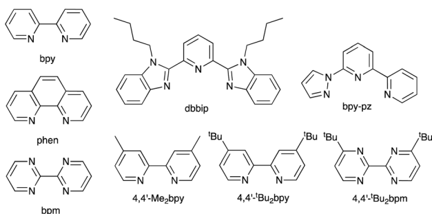
Scheme 3 Structures of bpy, phen, bpm, dbpip, bpy-pz, 4,4'-Me 2 bpy, 4,4'-tBu 2 bpy and 4,4'-di- tert -butyl-2,2'-bipyrimidine (4,4'-tBu 2 bpm).
